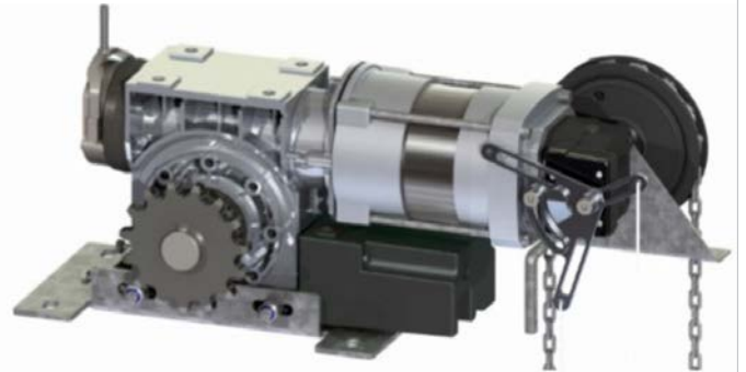
Haul Chain Mechanism (KE)
